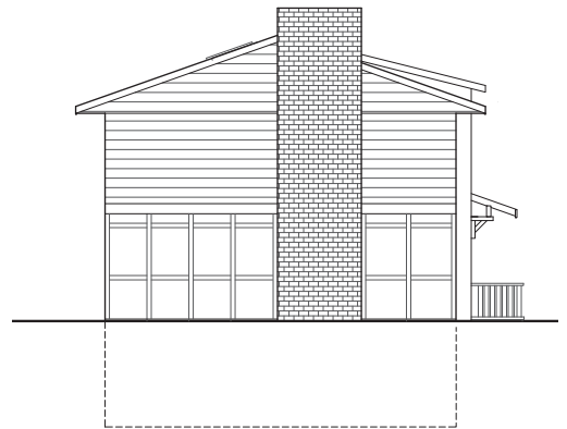
north elevation
